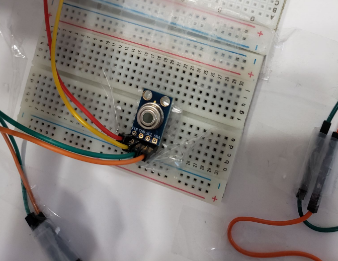
MLX90614 Temperature Sensor
