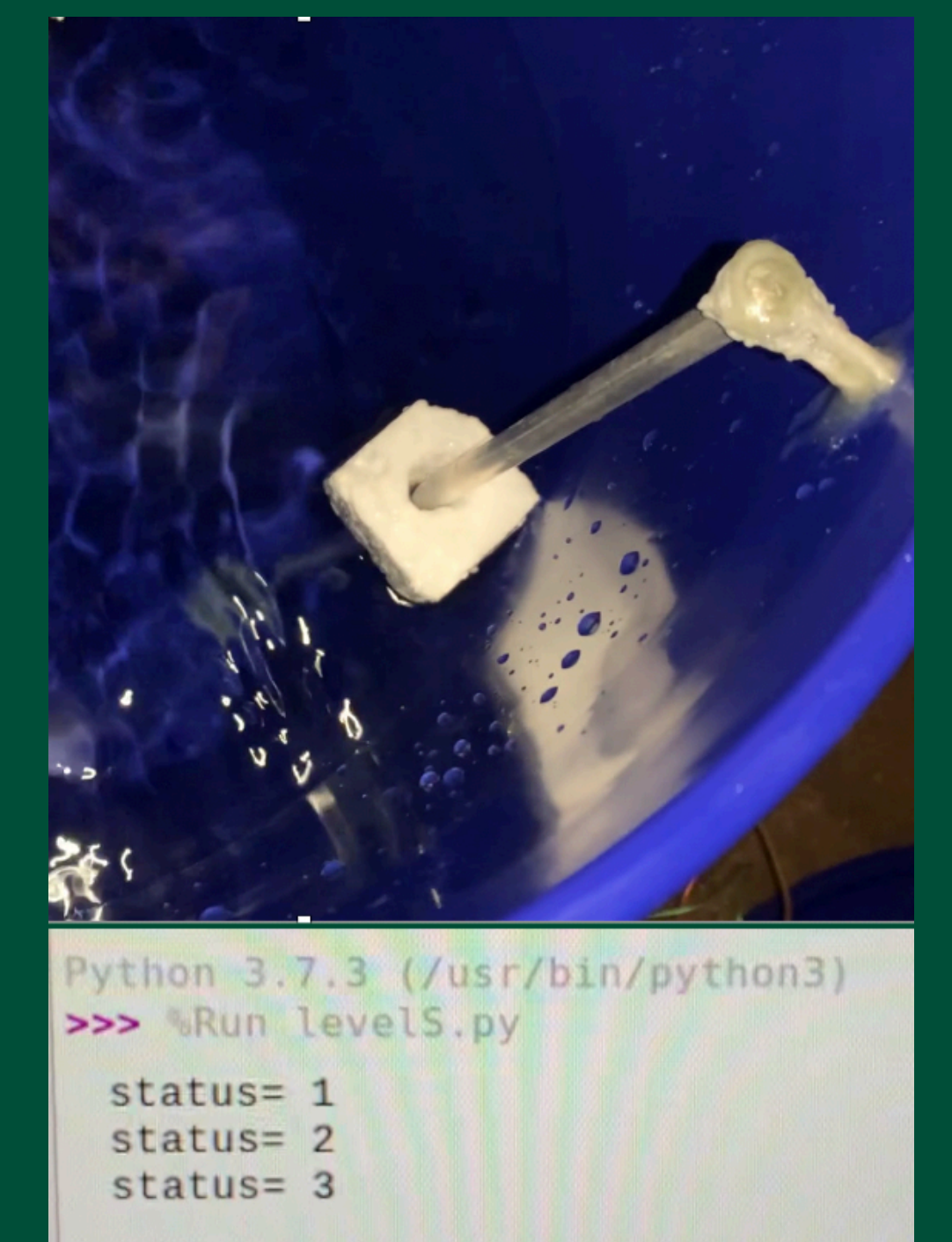
Figure 5: Using magnetic sensors to know the level of water in the tank.
